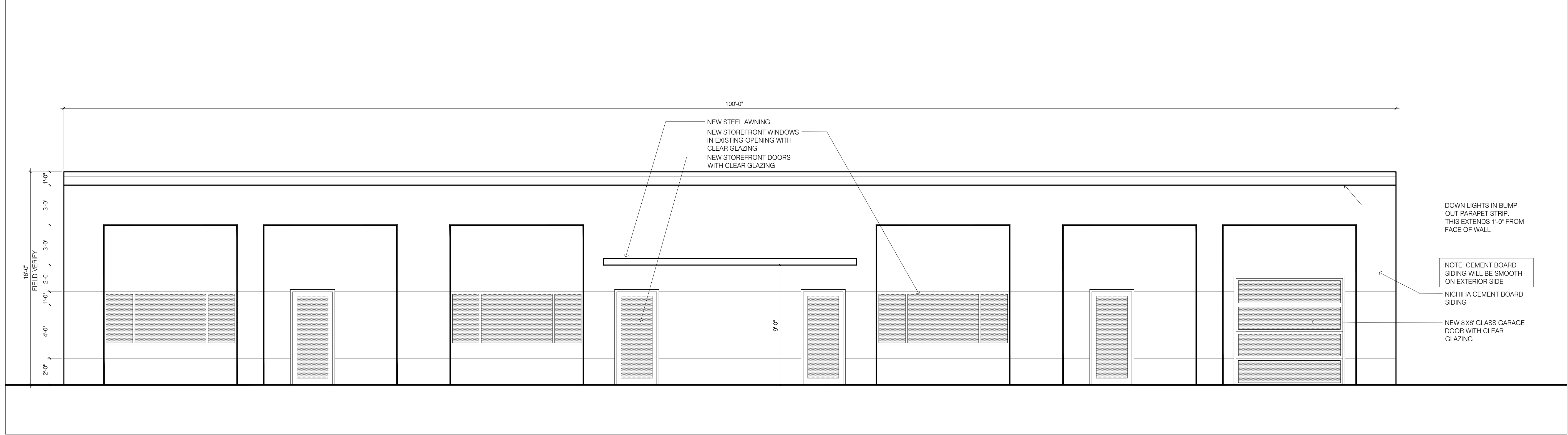
2 ELEVATION @ EXISTING BUILDING SCALE 1/4" = 1'-0"
