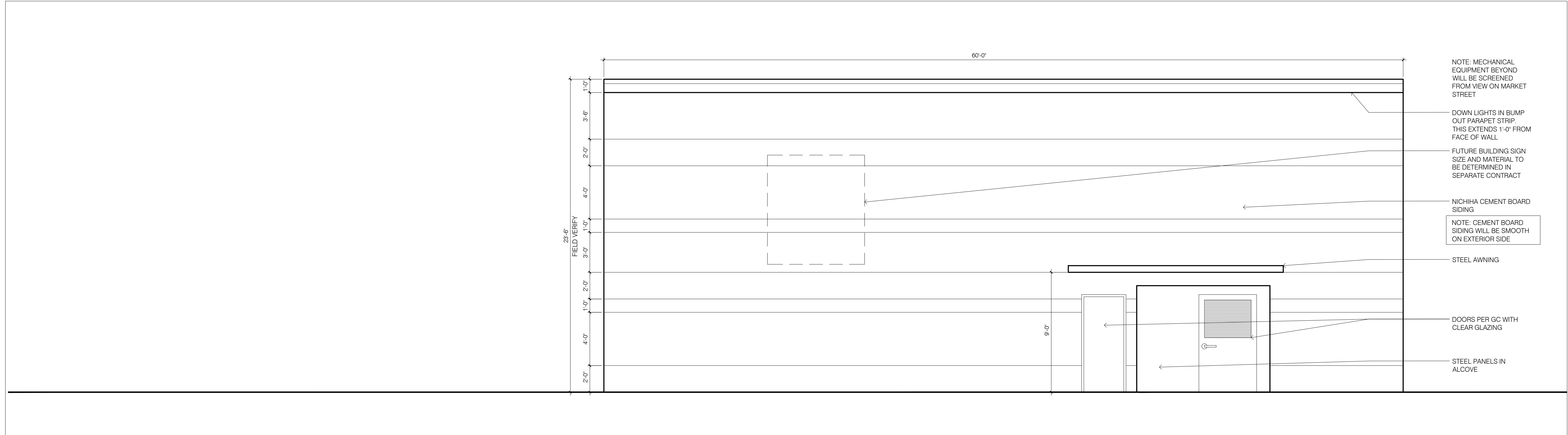
1 ELEVATION @ NEW BUILDING SCALE 1/4" = 1'-0"
